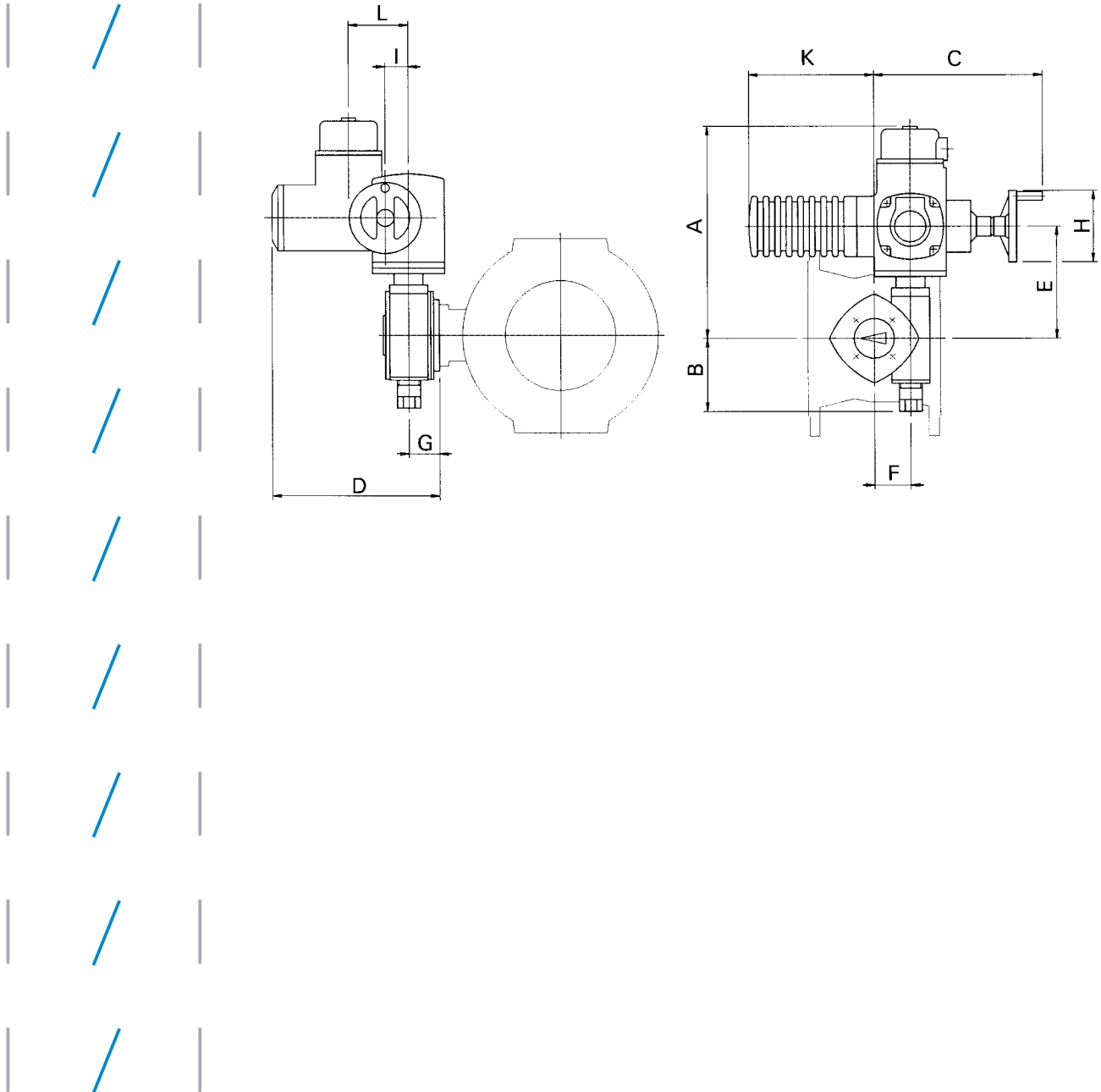
Worm Gear Type GS with multi-turn actuator SA
